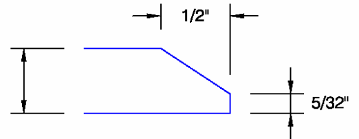
Section At Beveled Edge
