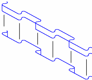
Interlocking Tab Detail
