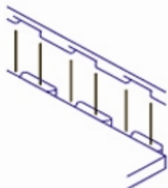
Interlocking Tab Detail
